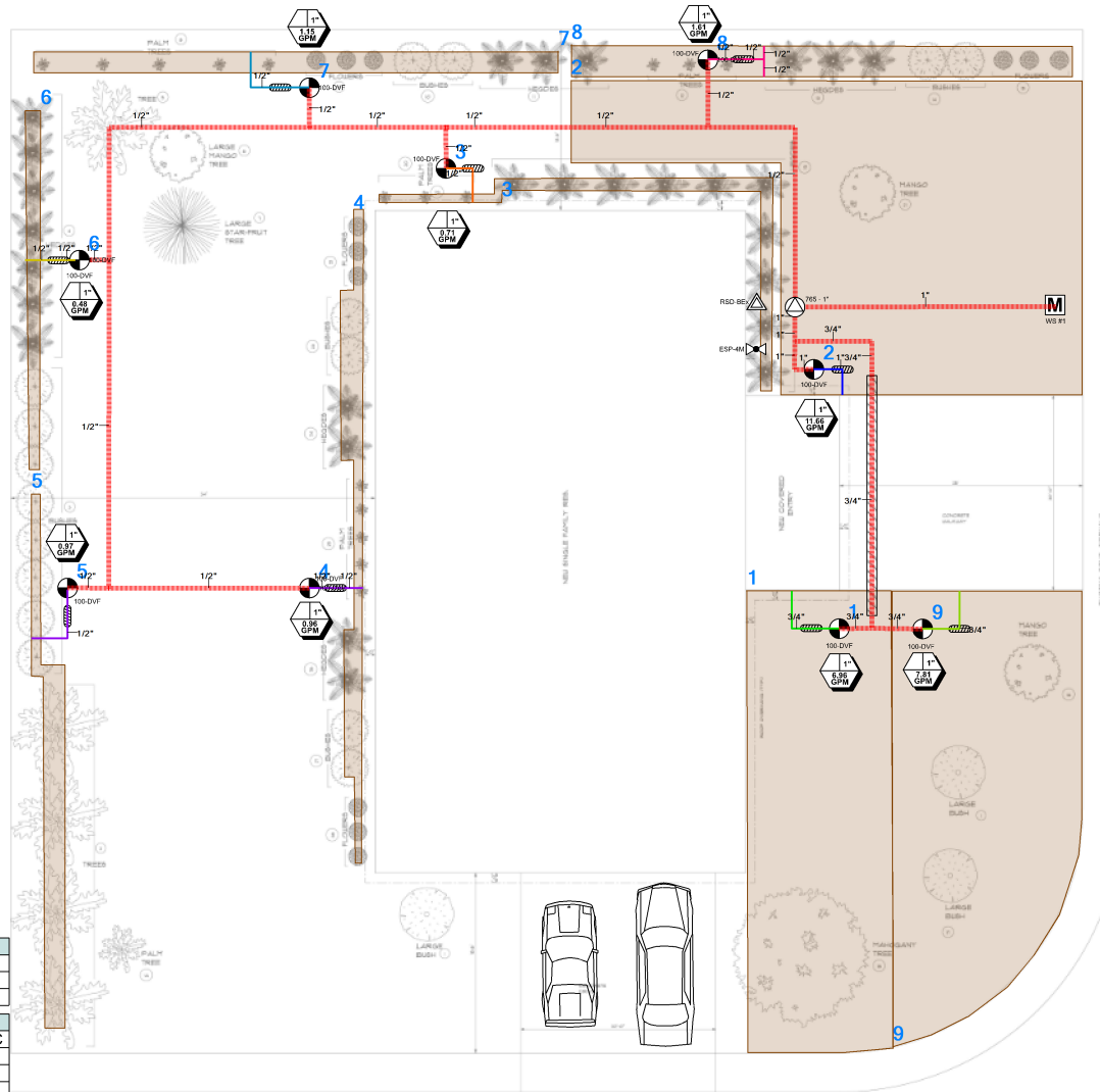
IRRIGATION PLAN
